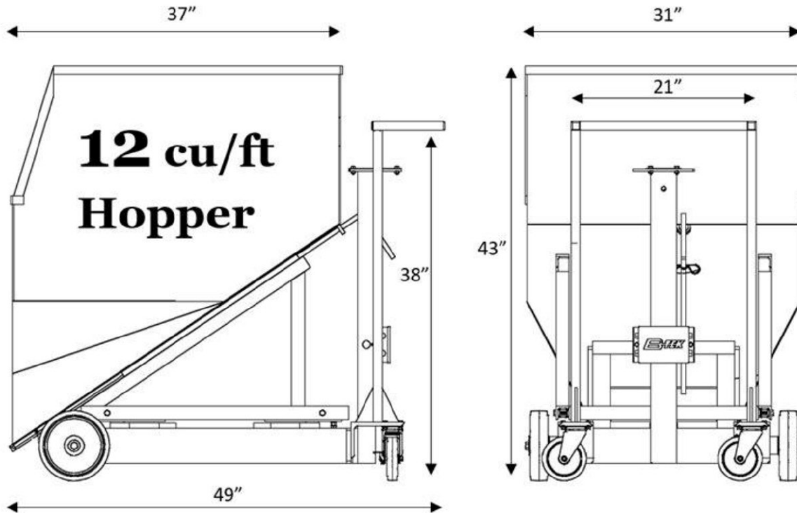
WEIGHING / LOAD RECEIVING ELEMENT BW-3024-IK-CS-WB (WEIGHT BUGGY)
