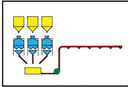
Blending ingredients for feed systems.
